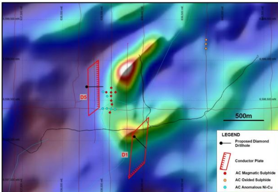
Figure 1: Area D Proposed Diamond Drillholes Testing D1 & D5 LF-MLTEM Conductors
