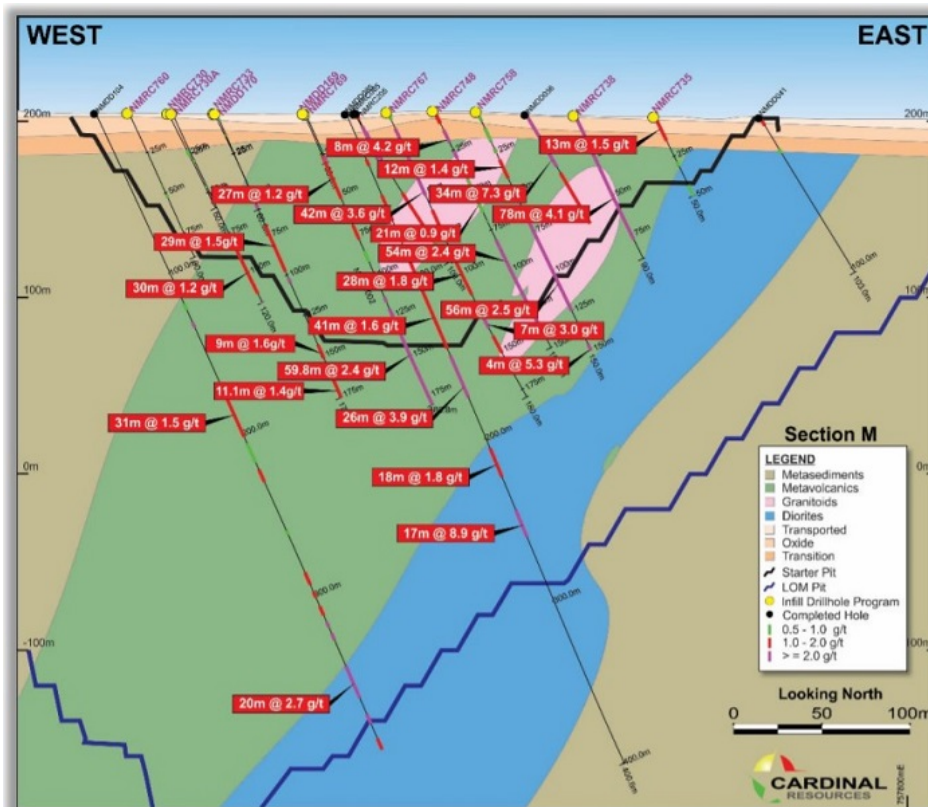
Cross Section showing downhole mineralised intersections of infill holes
