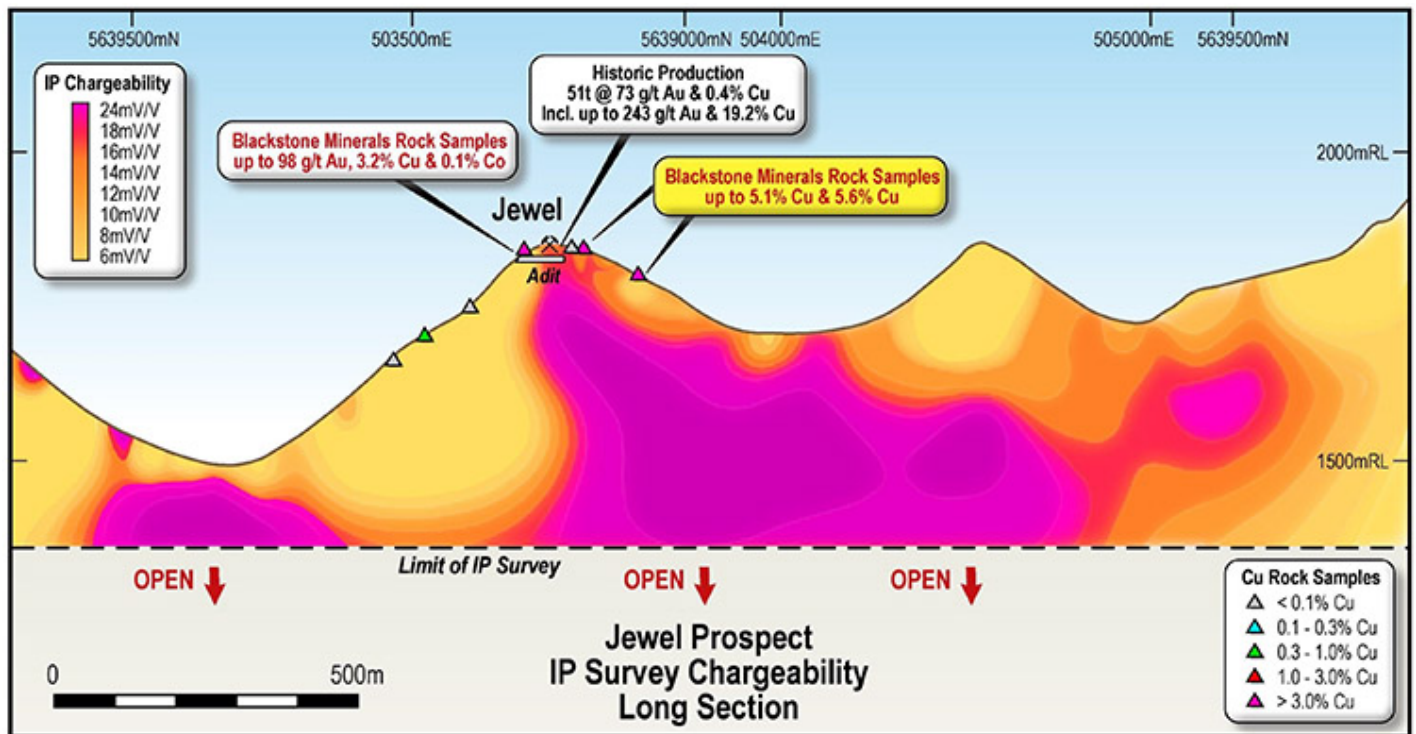
A long section schematic of chargeability isosurfaces and surface rock samples at Jewel
