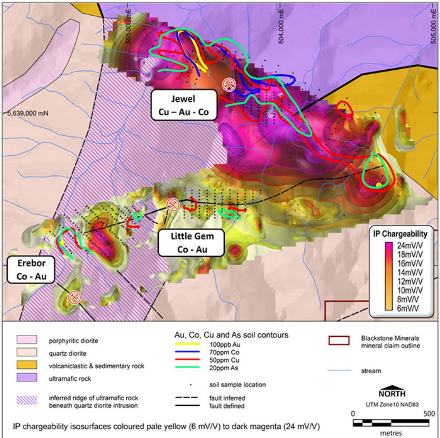
BC cobalt project plan with copper, gold and cobalt soil contours and IP chargeability isosurfaces
