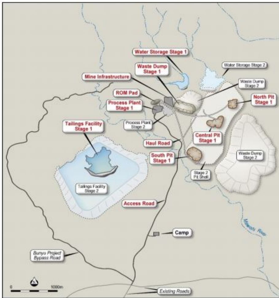
Stage 1 and Stage 2 Project layout.
